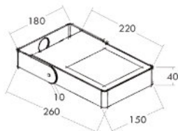
150 x 260 x H40mm FLAT EVO 3
