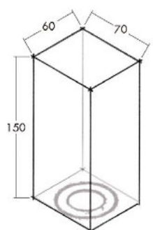
70 x 60 x H150mm BRICK 1
