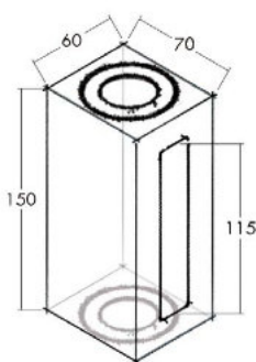
70 x 60 x H150mm BRICK 2-F
