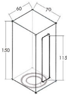
70 x 60 x H150mm BRICK 1-F
