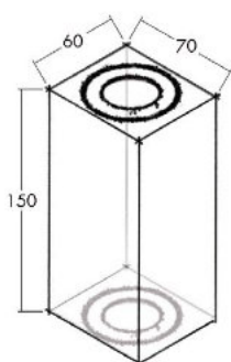
70 x 60 x H150mm BRICK 2
