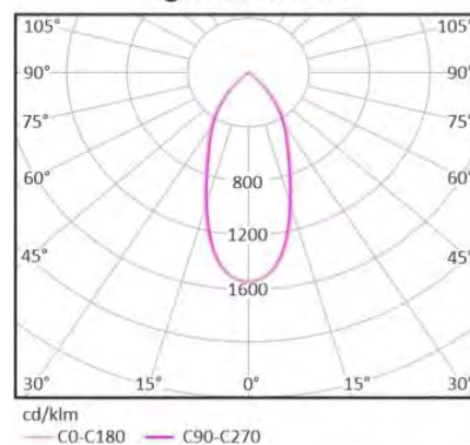
Light beam 36°
